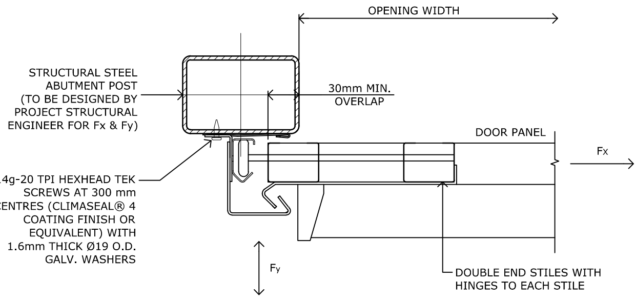
SECTION 1 1:5 PLAN OF TRACK FIXING TO STEEL ABUTMENT SUPPORT POST.
