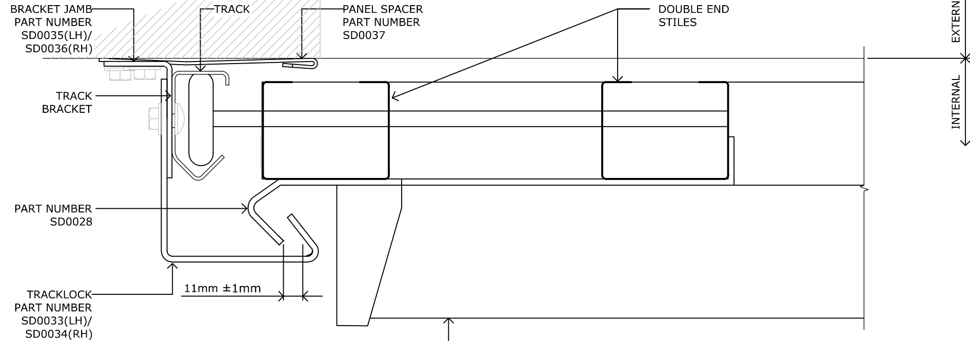
DETAIL B 1:2 TRACKLOCK SUPPORT BRACKET - PART PLAN (CROSS SECTION)
