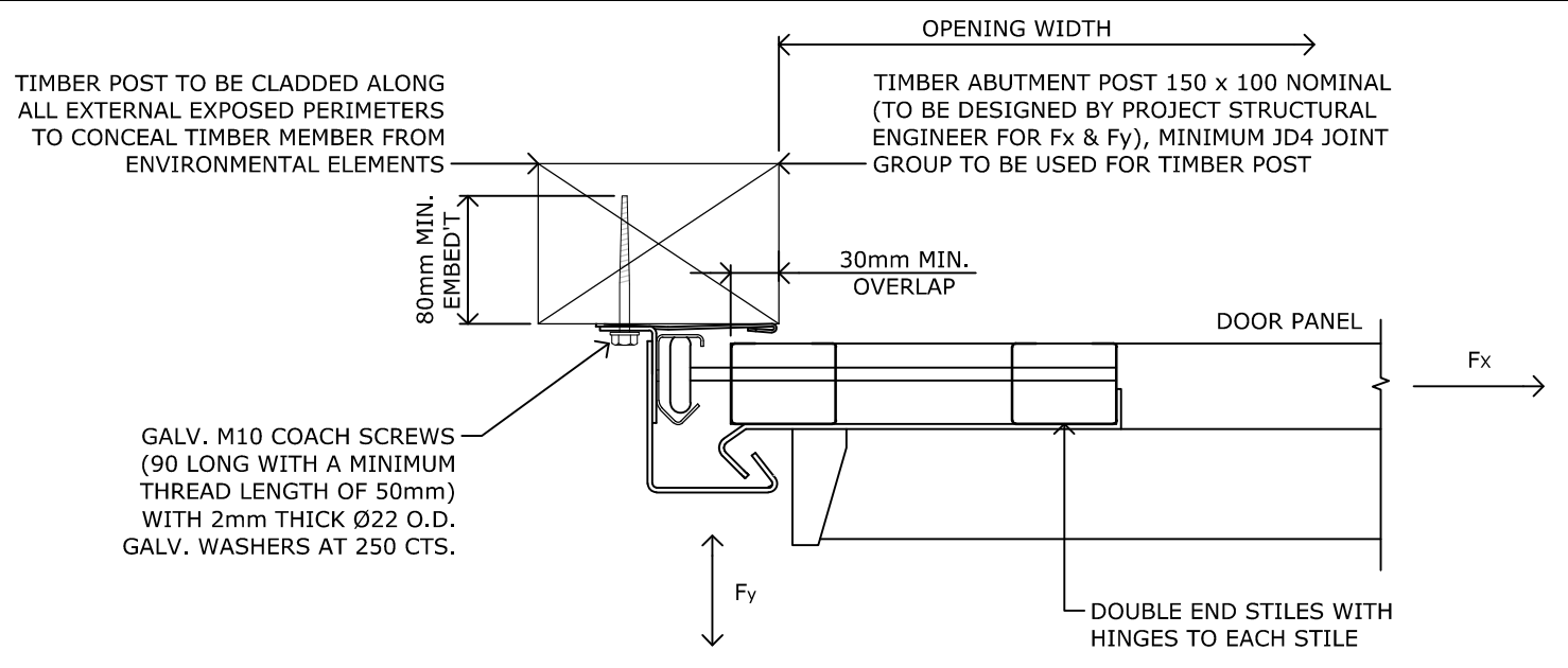
SECTION 1 1:5 PLAN OF TRACK FIXING TO TIMBER ABUTMENT SUPPORT POST.
