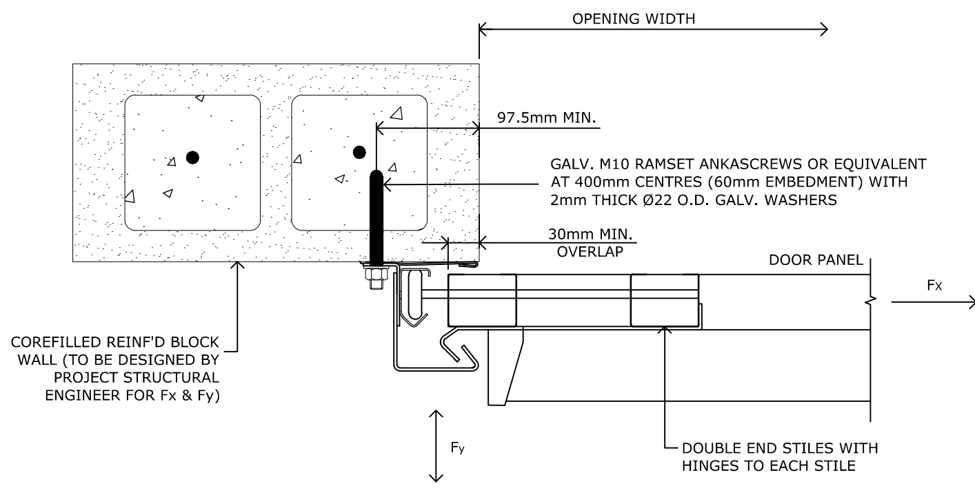
SECTION 1 1:10 PLAN OF TRACK FIXING TO REINFORCED COREFILLED BLOCKWORK ABUTMENT SUPPORTS.
